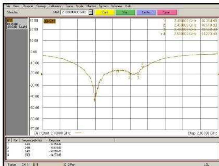
Return Loss
